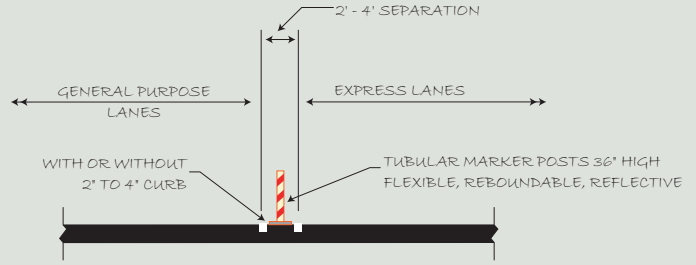
TUBULAR MARKER POSTS (SEMI-PHYSICAL SEPARATION)
