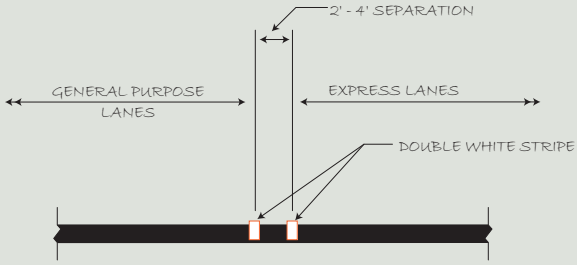
PAINT STRIPE SEPARATION (NO PHYSICAL SEPARATION)
