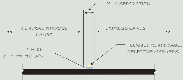
CURB & MARKER SEPARATION (SEMI-PHYSICAL SEPARATION)
